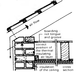
⑩ Pitched roof with timber beam ceiling
